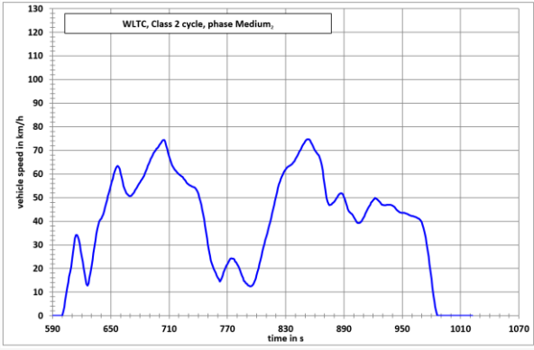
Figure A1/4 WLTC, Class 2 cycle, phase Medium 2
